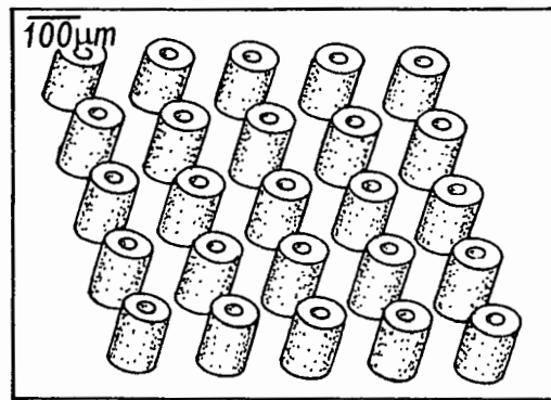
An array of silicon microneedles
